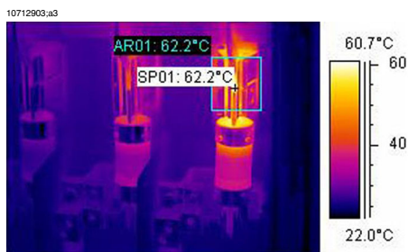
Figure 7.3 An infrared image of a fusebox where the maximum temperature is displayed
